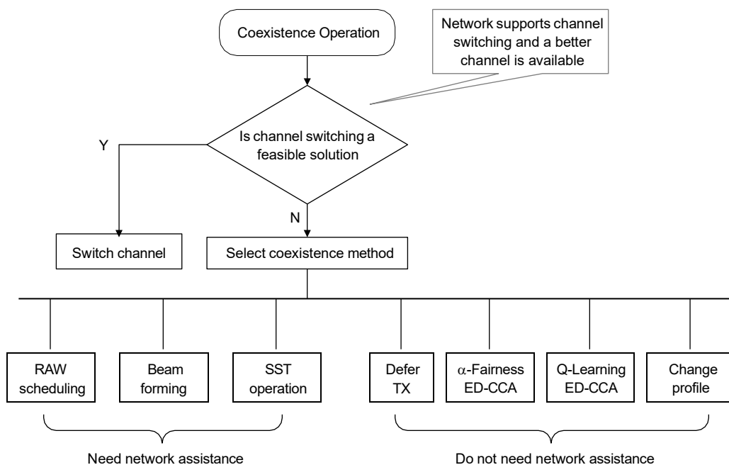
Figure 17—IEEE Std 802.11 S1G coexistence method selection
