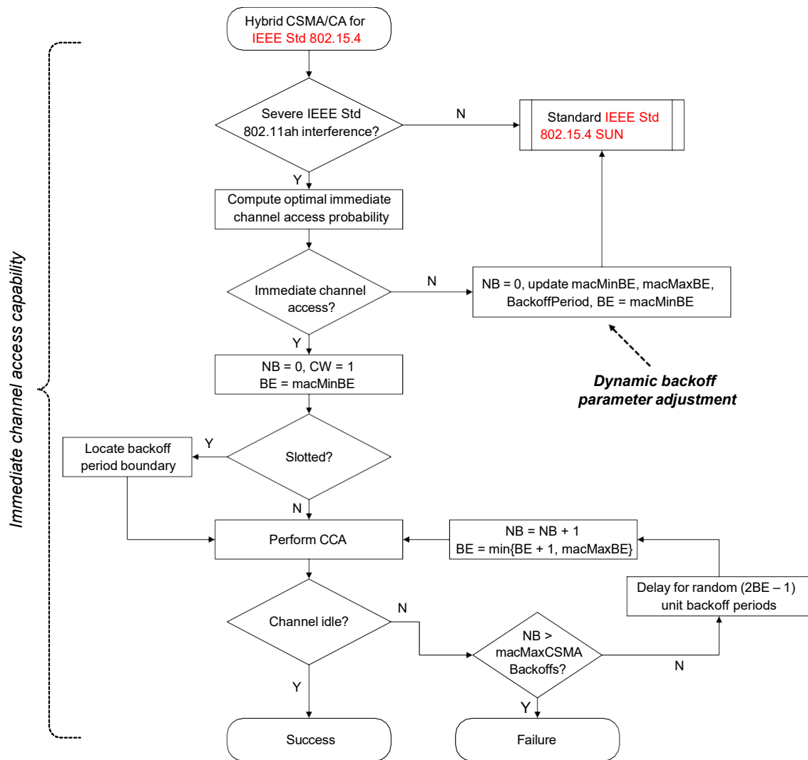
Figure 16—Hybrid CSMA/CA for IEEE Std 802.15.4 SUN
