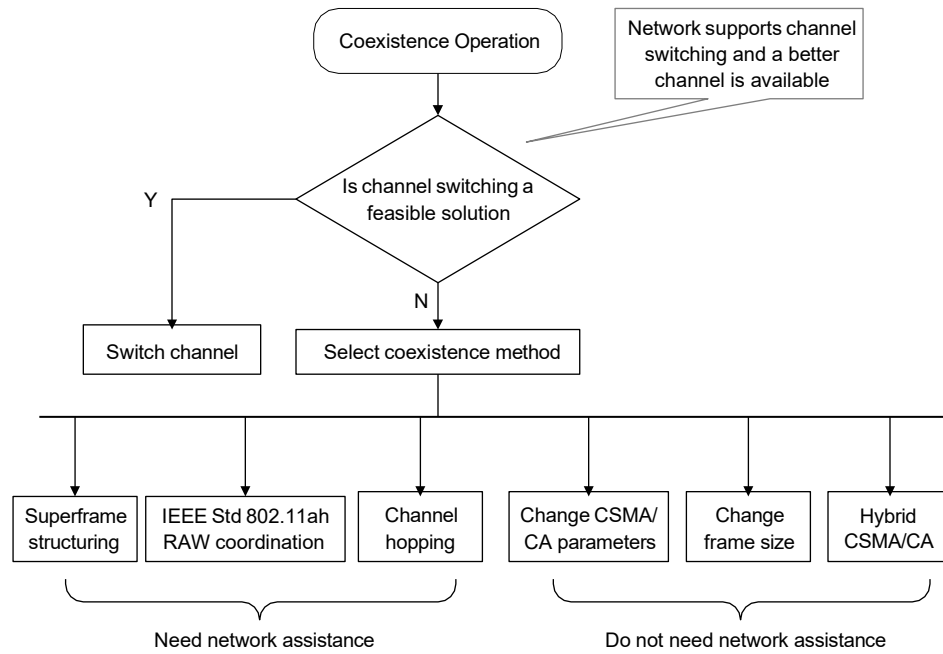
Figure 18—IEEE Std 802.15.4 SUN coexistence method selection
