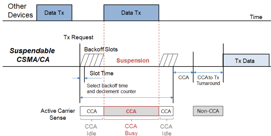
Figure 16b —Example of suspendable CSMA/CA behavior
