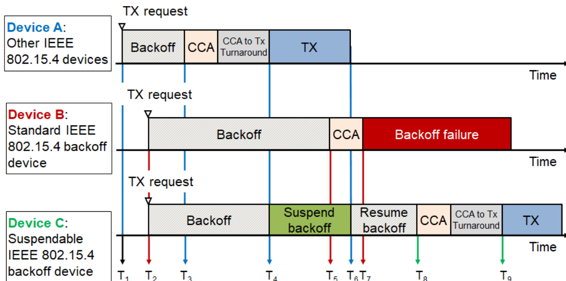
Figure 16a —Reduction of backoff failure by backoff suspension
