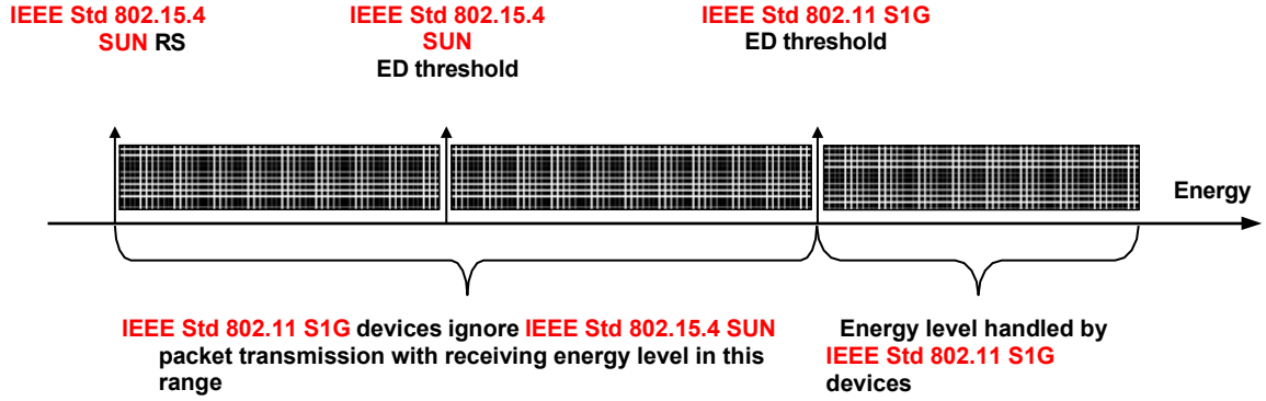
Figure 13—Interference caused by the higher ED threshold of IEEE Std 802.11 S1G
