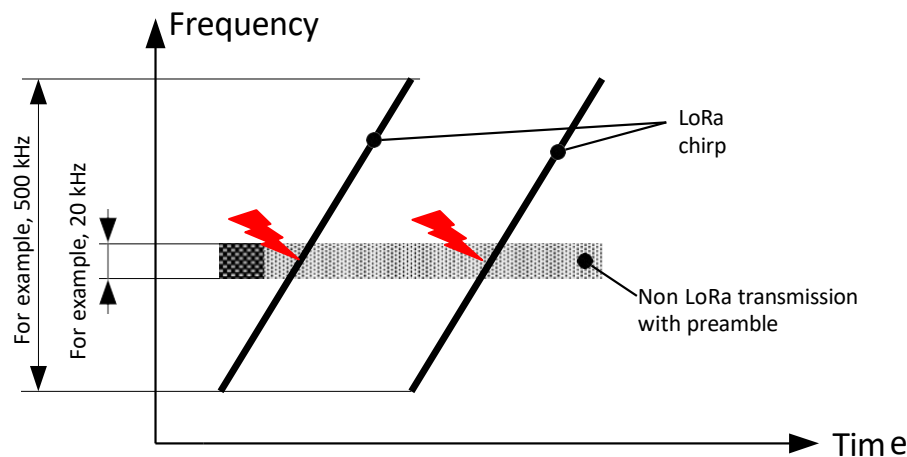
Figure 2—LoRa interference on other systems
