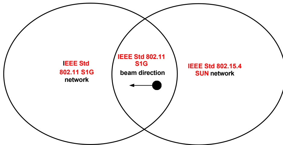
Figure 12—Coordinated beamforming
