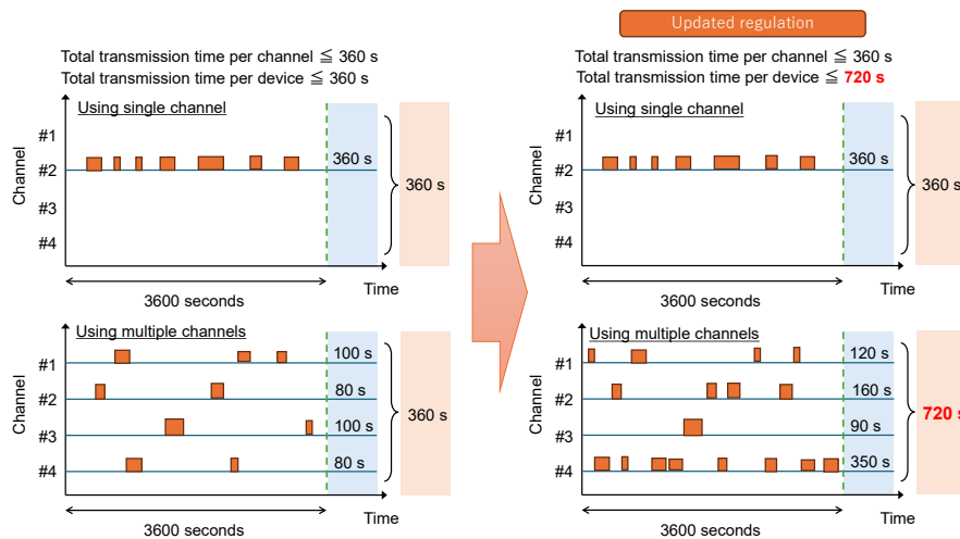
Figure 1a— Duty cycle update for active system
