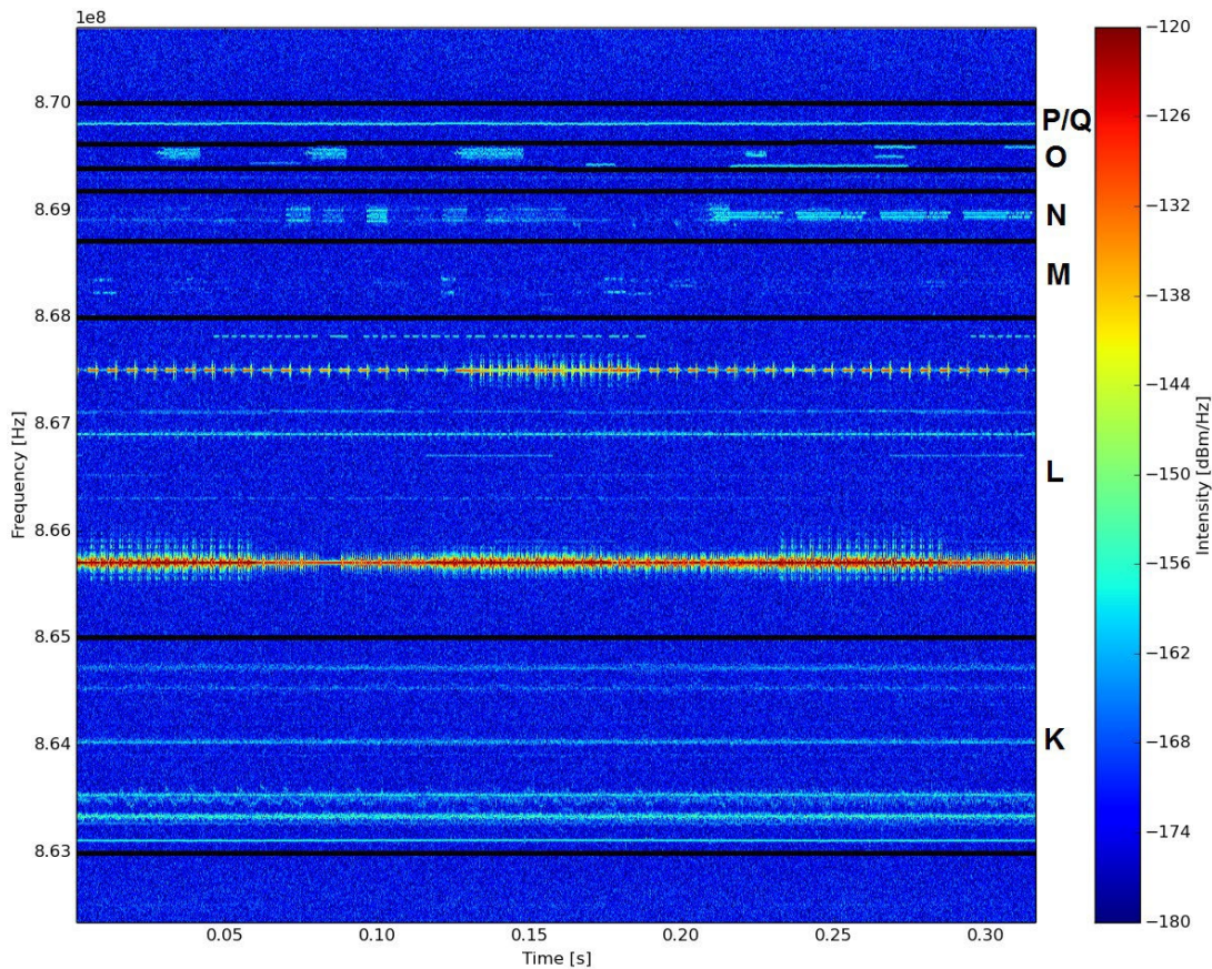
Figure 6—Measured SRD band from 863–870 MHz
