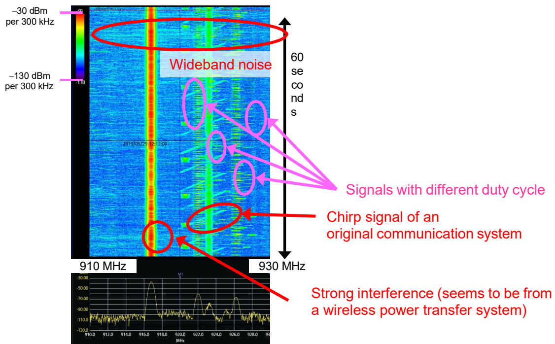
Figure 3—Spectrum utilization over 920 MHz band measured at a railway station
