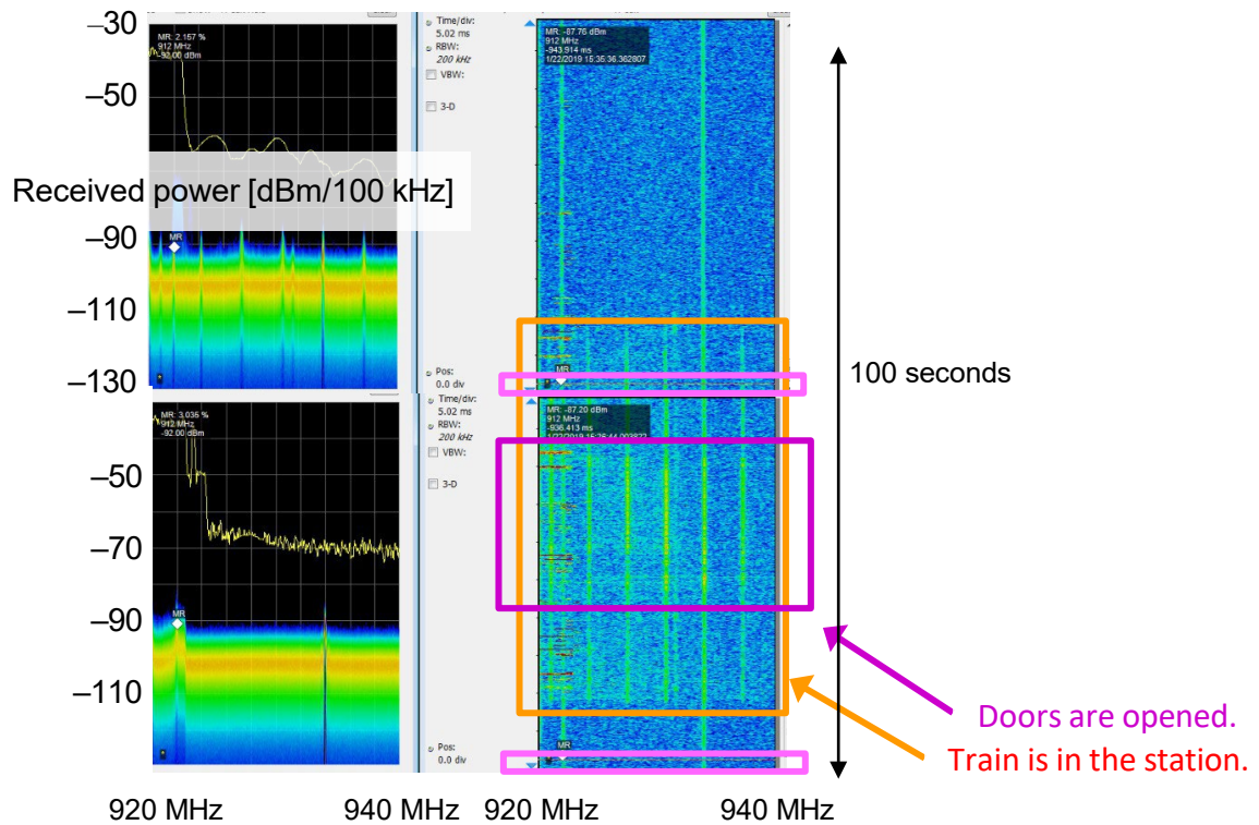
Figure 3—Spectrum utilization over 920 MHz band measured at a railway station
