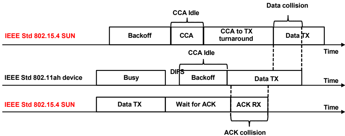
Figure 14—Interference caused by faster CSMA/CA of IEEE Std 802.11 S1G
