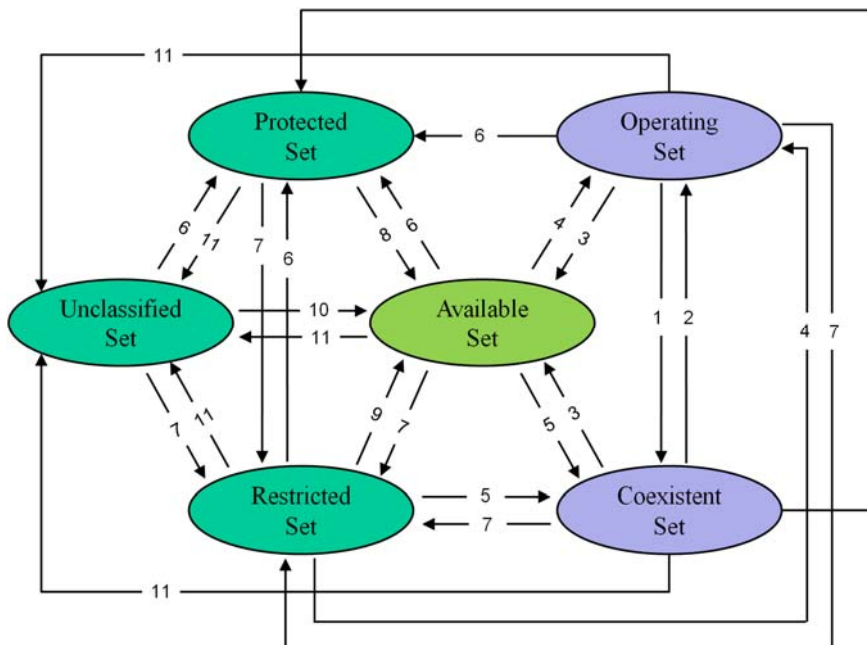
17 18 Figure 4 Channel set transition diagram
