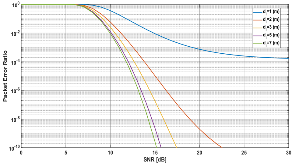
Figure 3—Packet Error Rate(PER) of Coexisting Two HBANs as a Funcion of SNR according to Distance between HBANs
