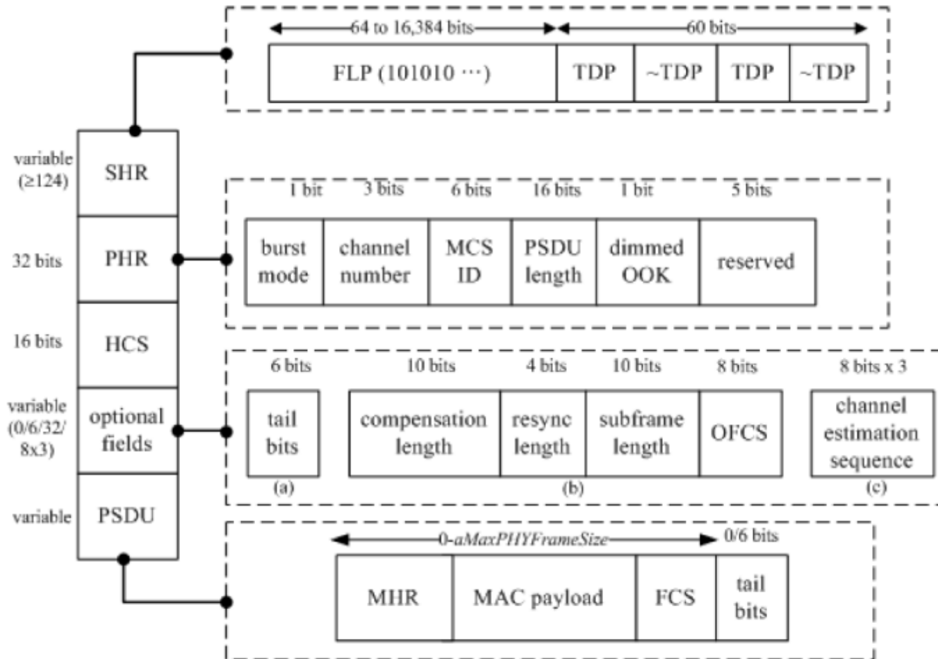
Figure 124—PPDU structure
