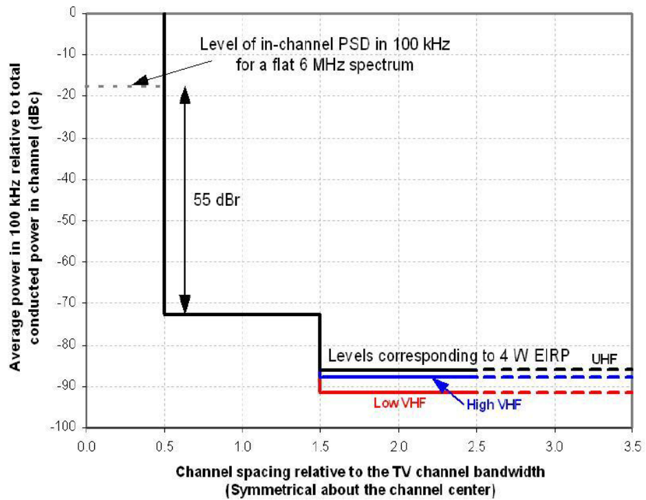
Figure 1: Frequency Mask Requirements for TV white Space Bands
