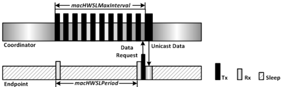
32 Figure 34sb—Unicast transmission in HWSL mode
