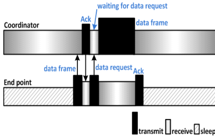
Figure 34sa—Basic LECIM LE mode operations
