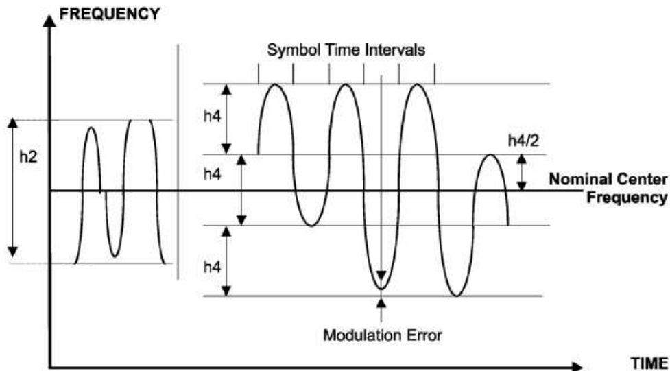
Figure 3—4-FSK modulation
