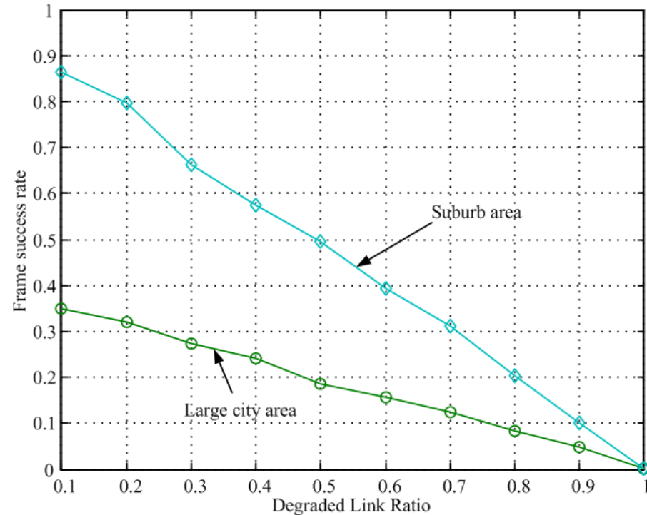
950MHz band
