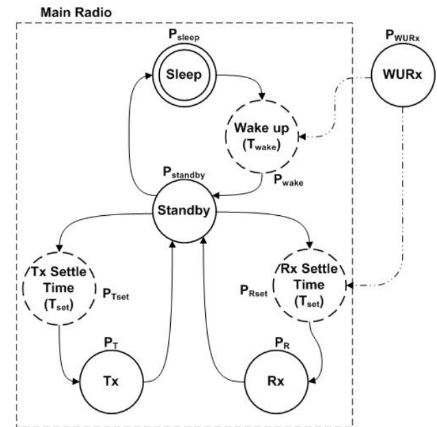
Radio Control State Diagram
