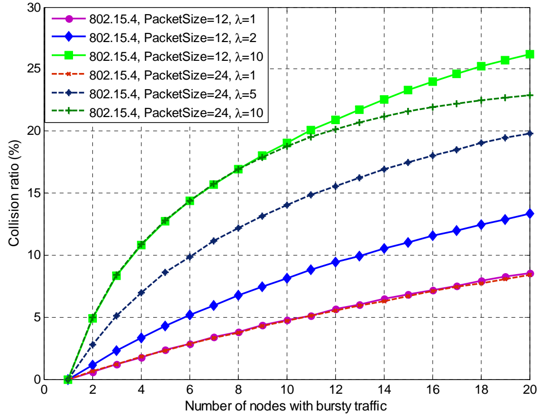
Collision Rate of CSMA-CA Mechanism
