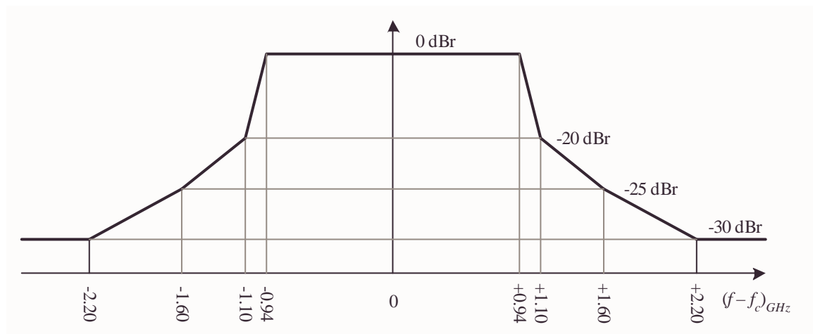
Figure 1—Transmit spectral mask
