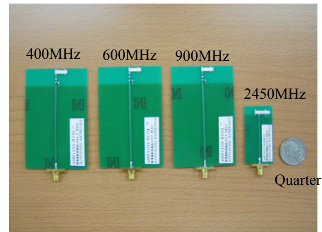
Chip antennas for frequency band of 400, 600, 900, and 2450MHz.
