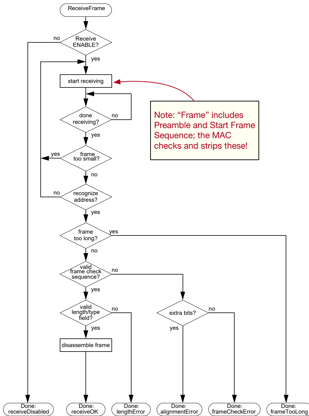
b) ReceiveFrame
