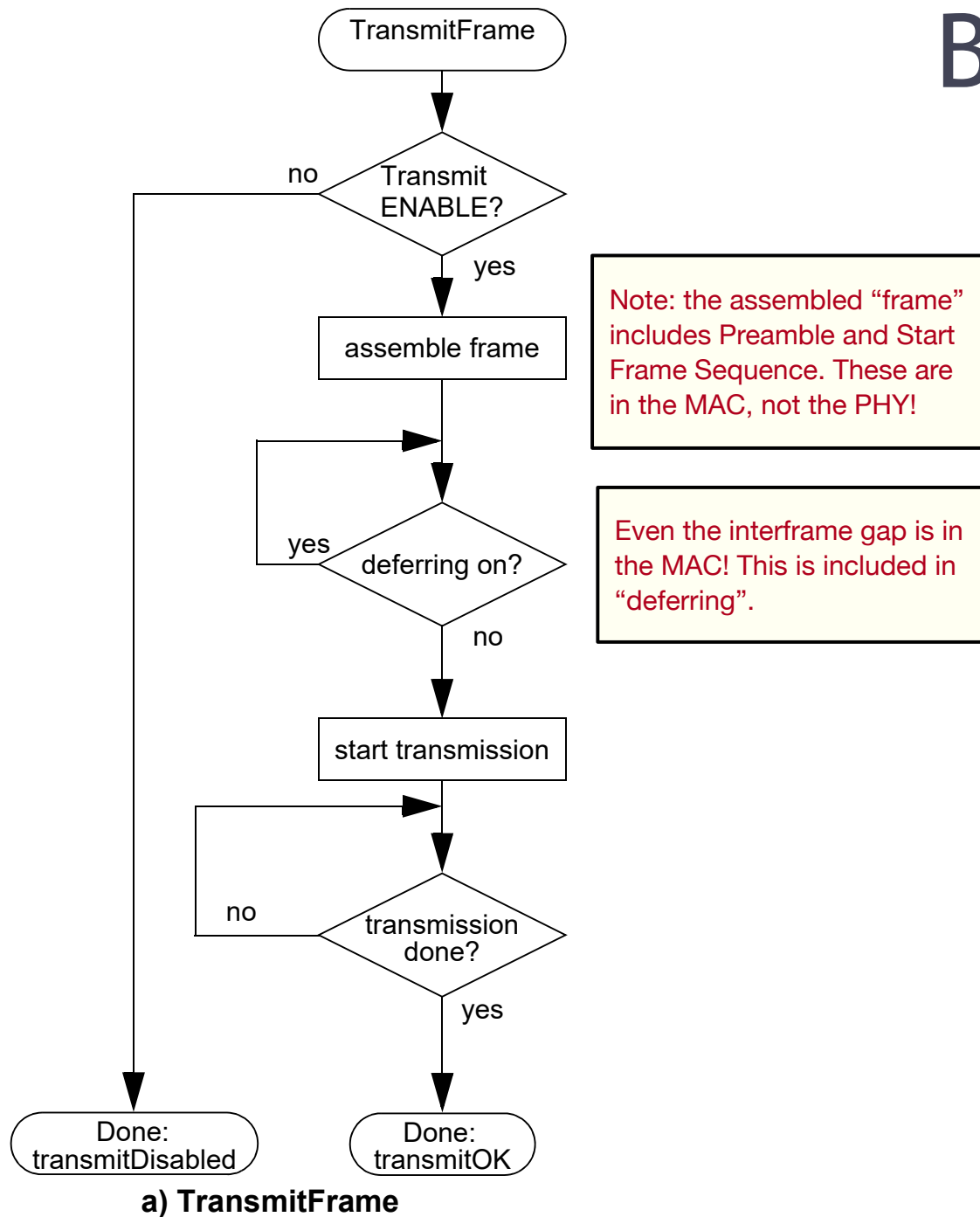
Figure 4A–2a—Control flow summary
