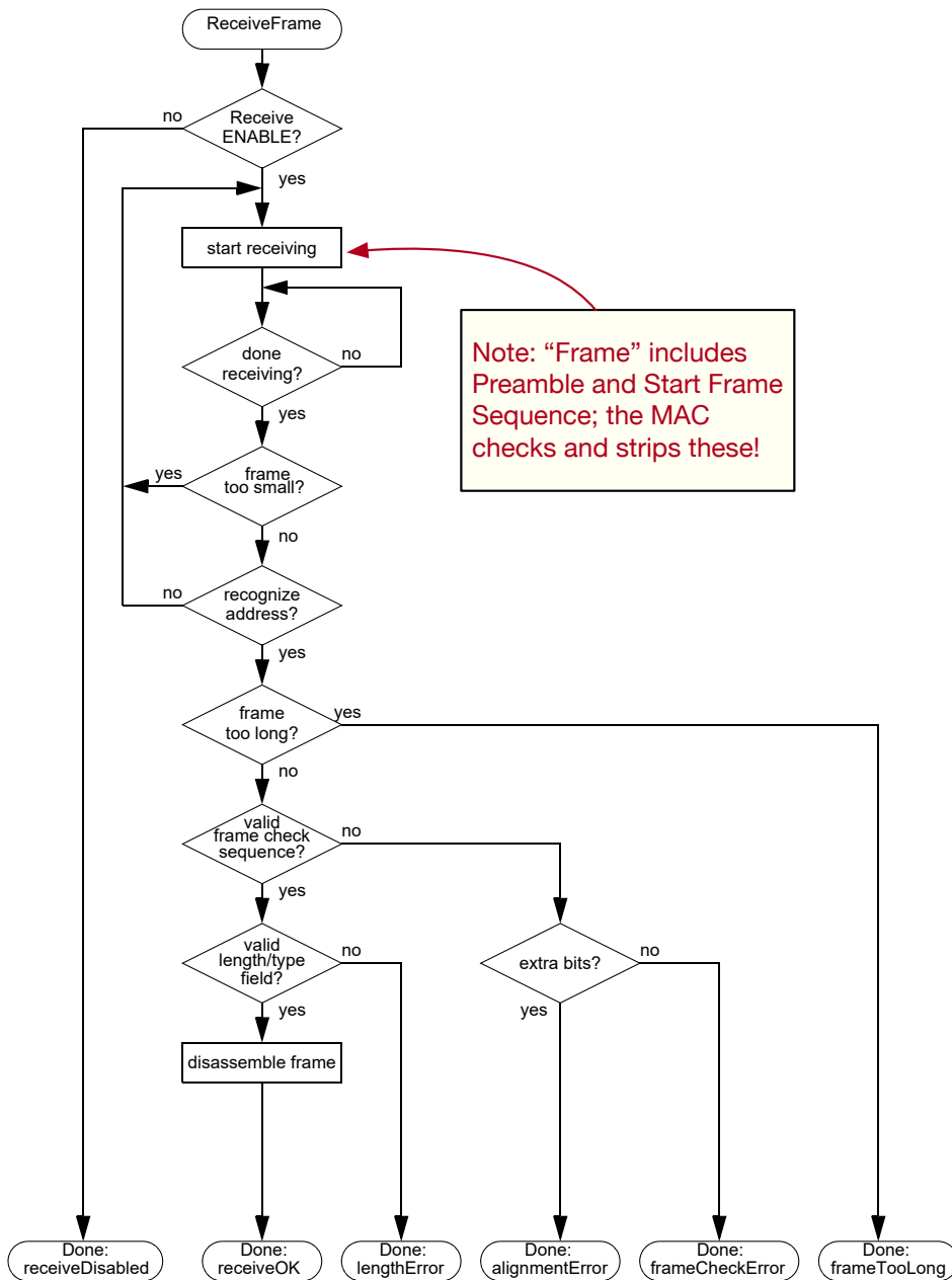
b) ReceiveFrame
