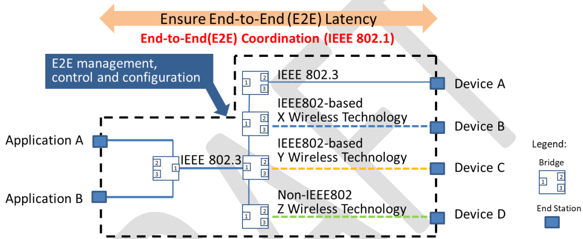
11 12 Figure 2 Example of Network Topology in Factory Environment
