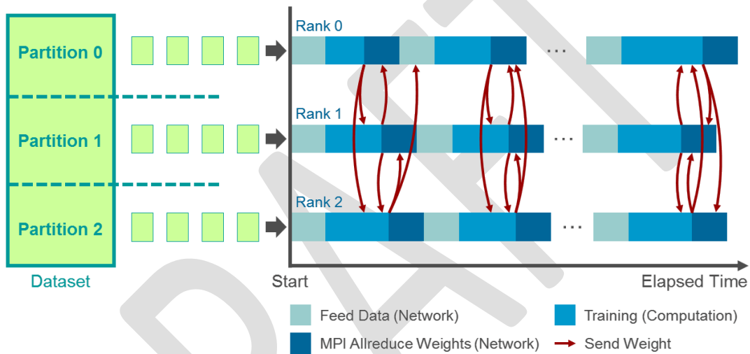
15 16 17 18 19 20 21 22 23 24 25 26 27 28 29 30 31 32 33 34 Figure 2 – Deep Learning Training
