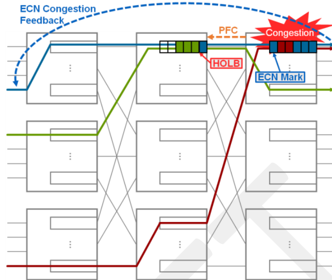
Figure 10 – PFC Head-of-Line Blocking
