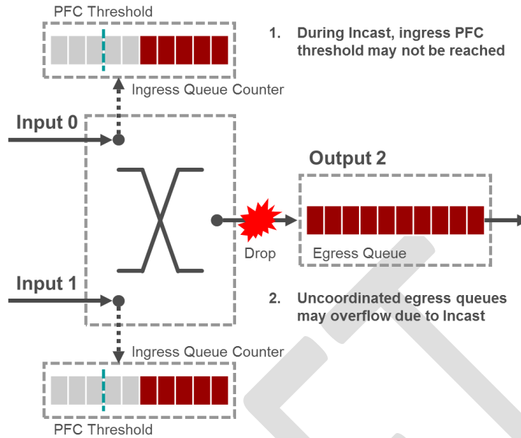
Figure 11 – Switch Packet Loss
