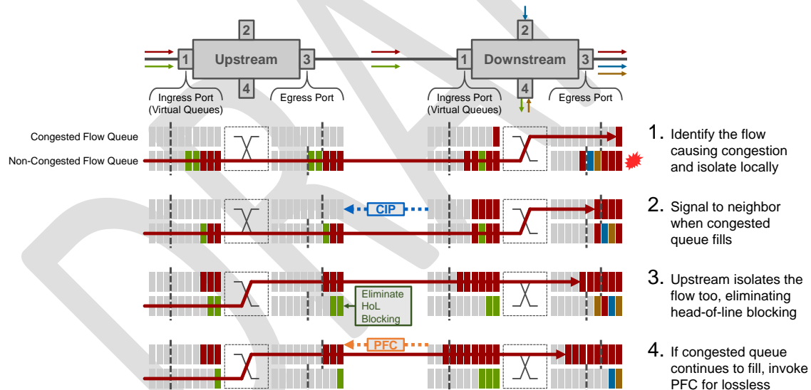
Figure 12 – Dynamic Virtual Lanes
