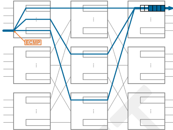
Figure 7 – ECMP Load Balancing
