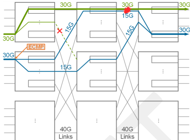
Figure 9 – ECMP Load Balancing Collisions
